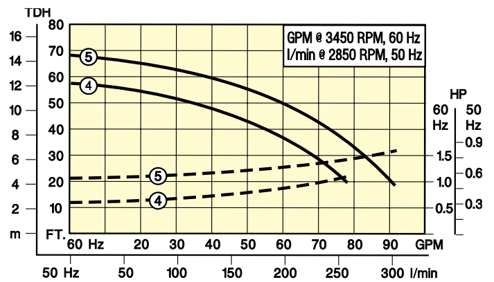
MODEL EO1¼
