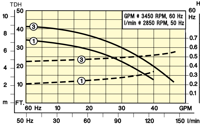
MODEL EO1
